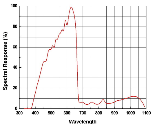
Fig.5 Spectral Response
