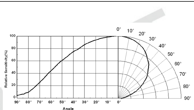
Fig 12 Relative Sensitivity vs. Angle
