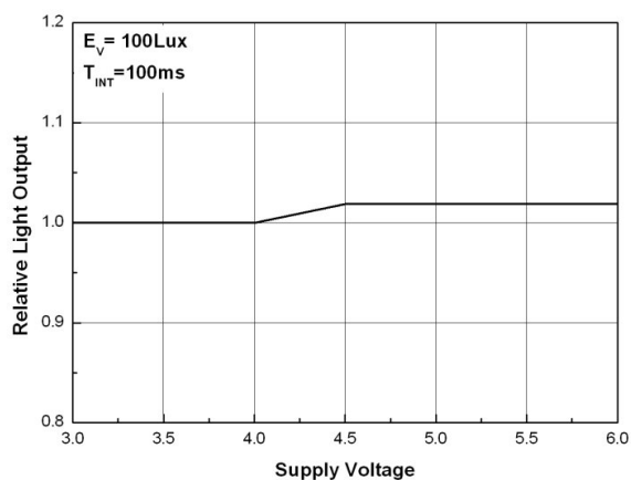
Fig 7 Light Counts vs. Supply Voltage (Ta=25 °C)
